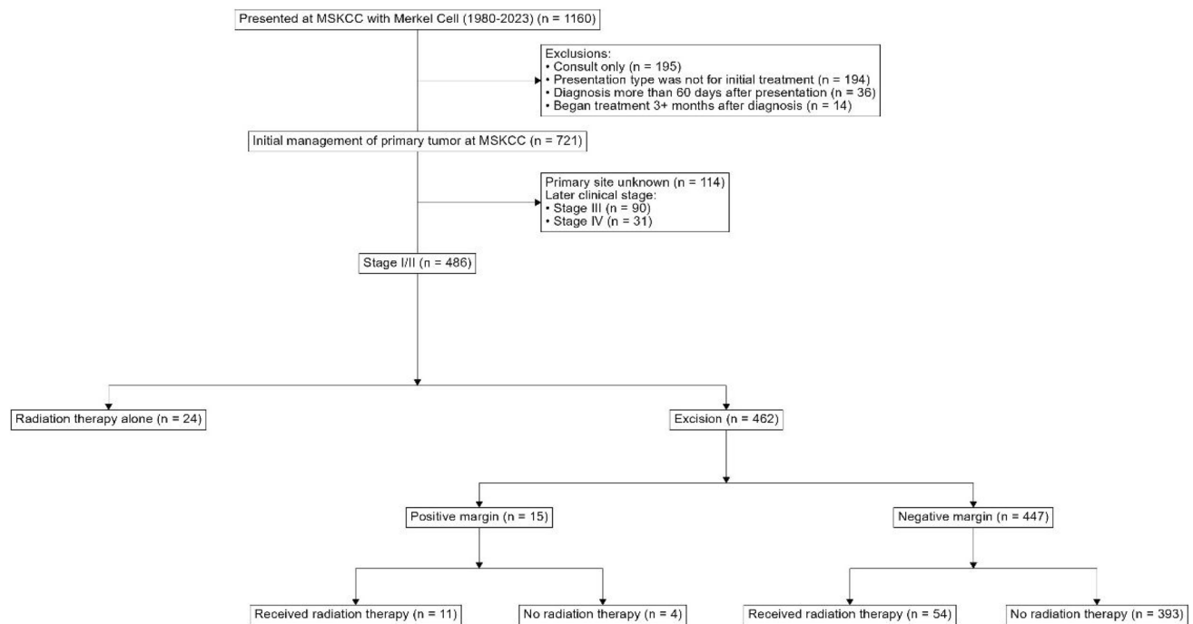
FIG. 1 Enrollment diagram
